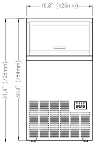
ADA-Height Configuration
