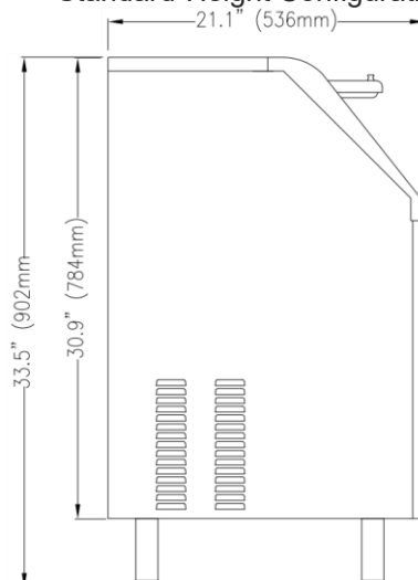
Standard-Height Configuration
