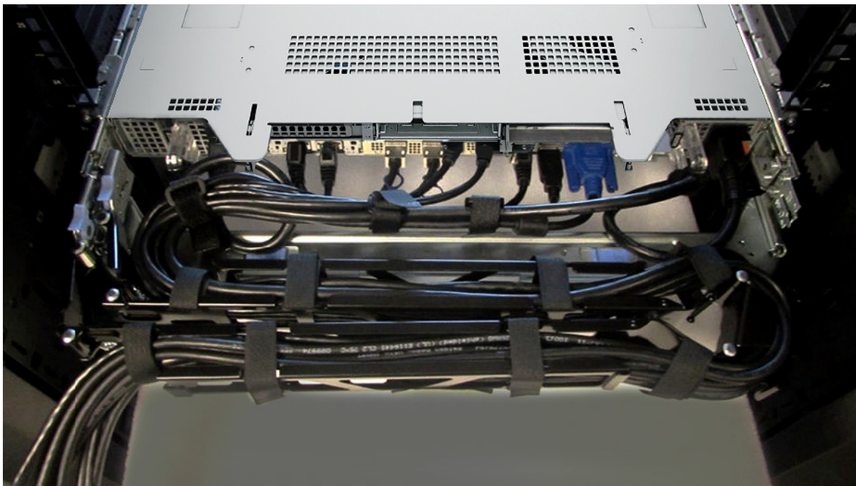
Figure 49. CMA Cabling
