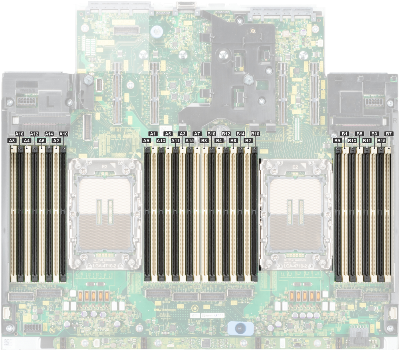
Figure 22. Memory channels
