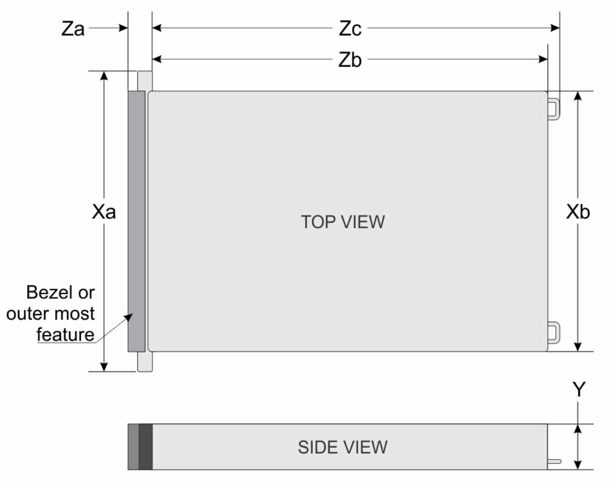
Figure 51. Chassis dimensions
