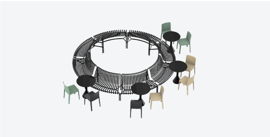
Park Dining Bench | 8 x OUT | Inner Ø260 cm | Outer Ø420 cm
