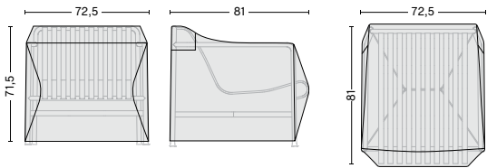
FOR LOUNGE CHAIR LOW Width 72,5 cm Depth 81 cm Height 71,5 cm
