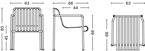
PALISSADE DINING ARMCHAIR Width 63 cm Depth 66 cm Height 80 cm Seat height 45 cm Seat depth 44 cm Weight 11 kg
