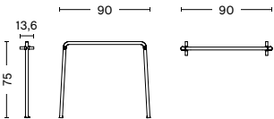
PALISSADE MIDDLE LEG Width 90 cm Depth 13,5 cm Heigth 75 cm Weight 3,48 kg
