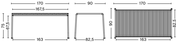
PALISSADE TABLE Length 170 cm Width 90 cm Height 75 cm Weight 31,55 kg
