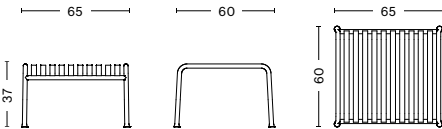
PALISSADE OTTOMAN Width 65 cm Depth 60 cm Height 37 cm Weight 9 kg
