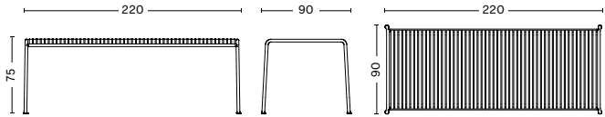
PALISSADE TABLE Length 220 cm Width 90 cm Height 75 cm Weight 37,8 kg
