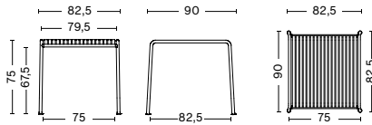
PALISSADE TABLE Length 82,5 cm Width 90 cm Height 75 cm Weight 17,9 kg
