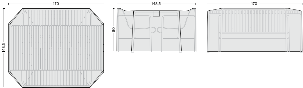
FOR TABLE INCL. 2 PCS DINING ARMCHAIR Length 170 cm Width 148,5 cm Height 80 cm
