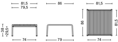
PALISSADE LOW TABLE Length 81,5 cm Width 86 cm Heigth 38 cm Weight 17,63 kg
