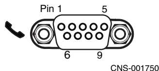
Figure 36 Control Station modem (DB-9) plug connector
