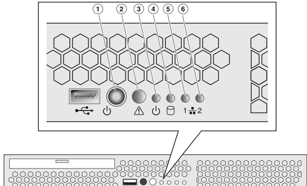
Figure 13 VNX5700 platform Control Station switch and LEDs
