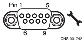
Figure 35 Control Station serial console (DB-9) plug connector
