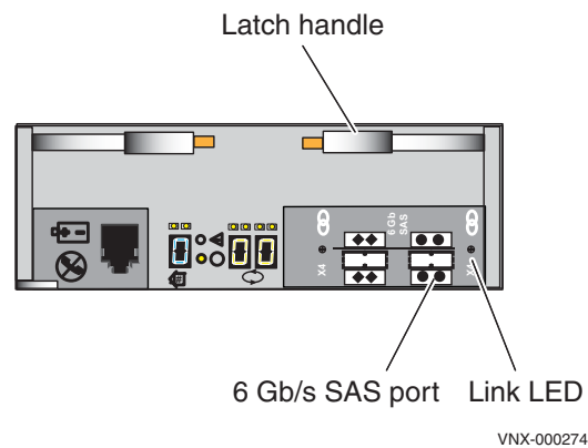
Figure 66 6-Gb/s SAS port LED
