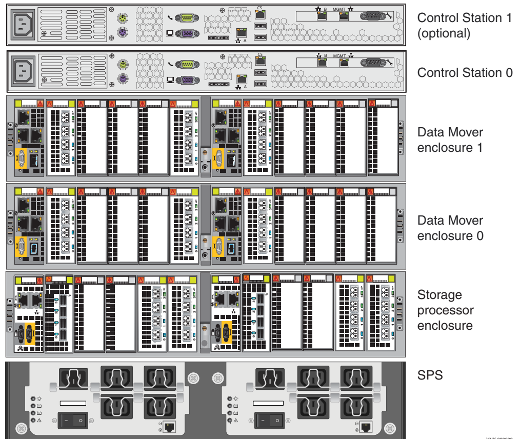
Figure 5 Example of a Block and File (Unified) VNX5700 platform using a 2U SPS (rear view)
