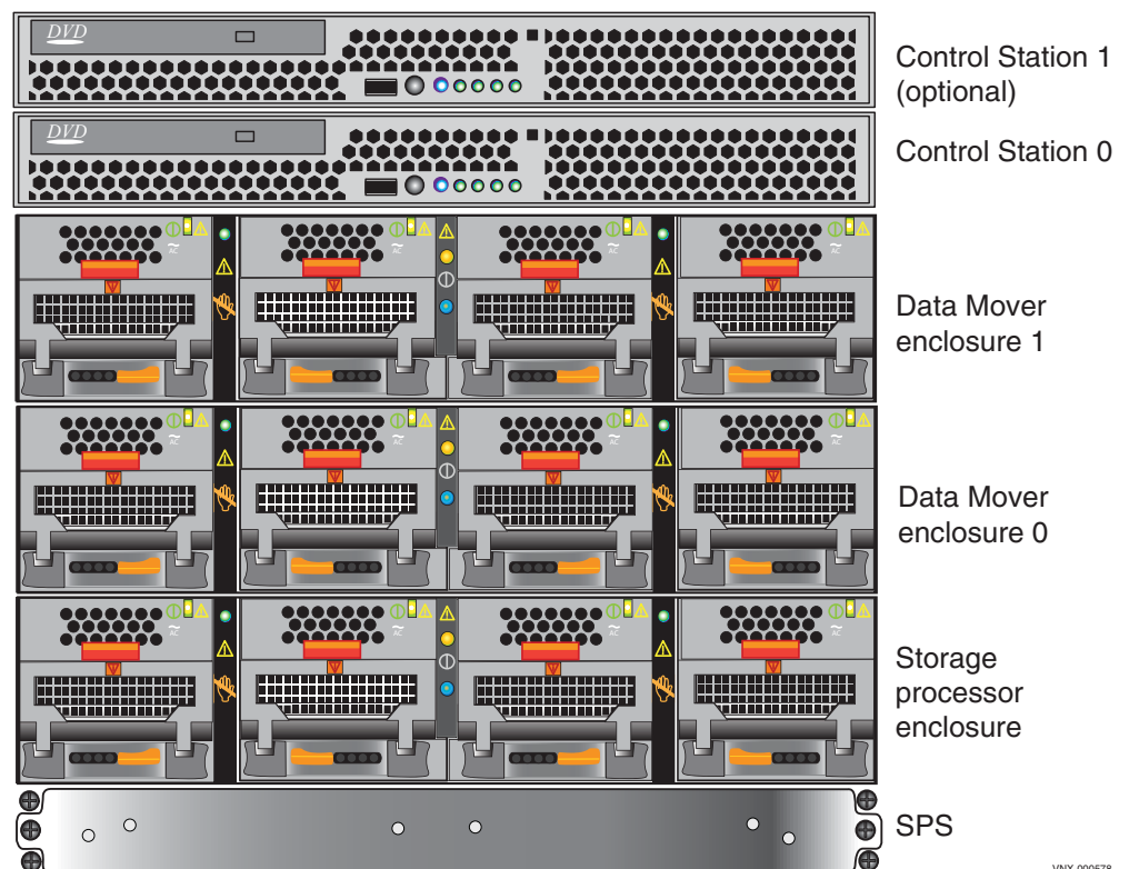
Figure 2 Example of a Block and File VNX5700 platform (front view)
