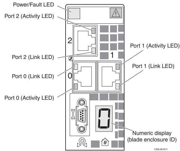
Figure 29 Data Mover management module LEDs
