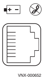
Figure 82 ICM RJ-12 port
