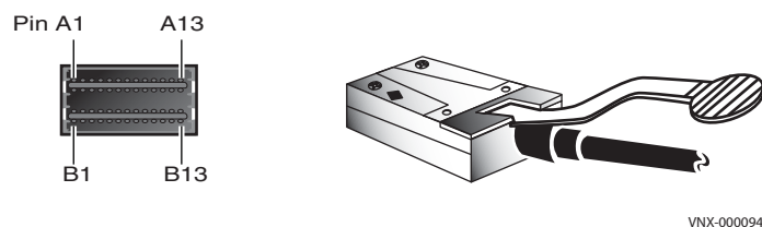
Figure 80 6-Gb/s SAS port and cable connector
