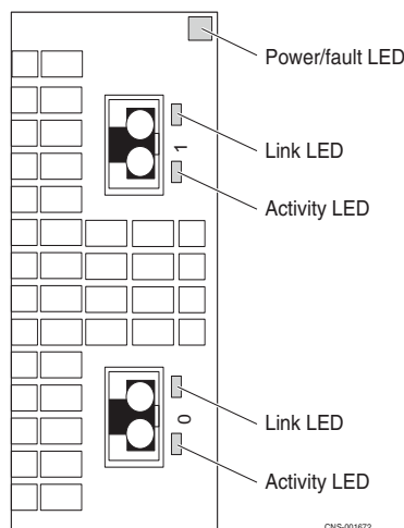
Figure 42 Two-port 10-Gb/s optical I/O module LEDs
