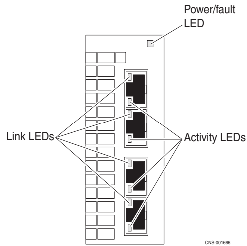
Figure 50 Four-port 1-Gb/s copper I/O module LEDs
