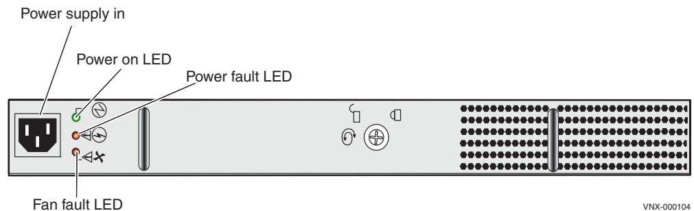
Figure 57 Example of a 3U, 15 (3.5-inch) DAE AC power supply/cooling module power in (recessed) connector (plug) and status LEDs
