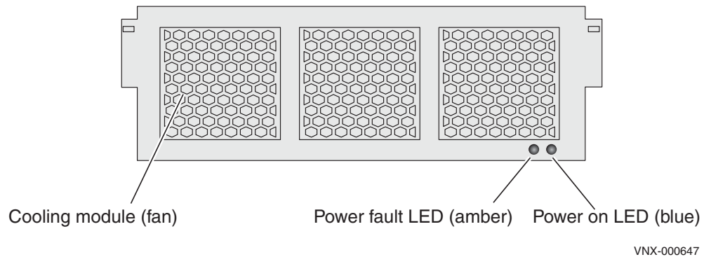
Figure 77 4U, 60 DAE (front view)
