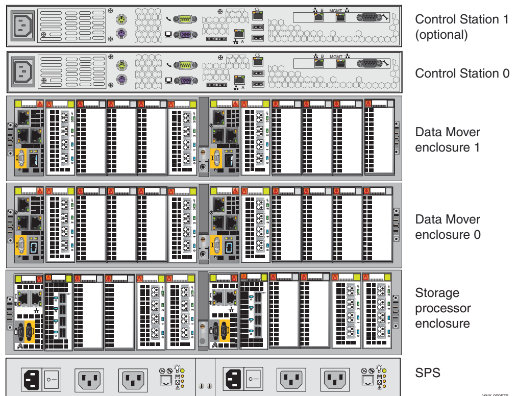
Figure 3 Example of a Block and File VNX5700 platform (rear view)
