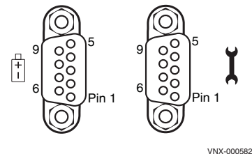
Figure 25 SP Management module serial console (DB-9) socket connectors
