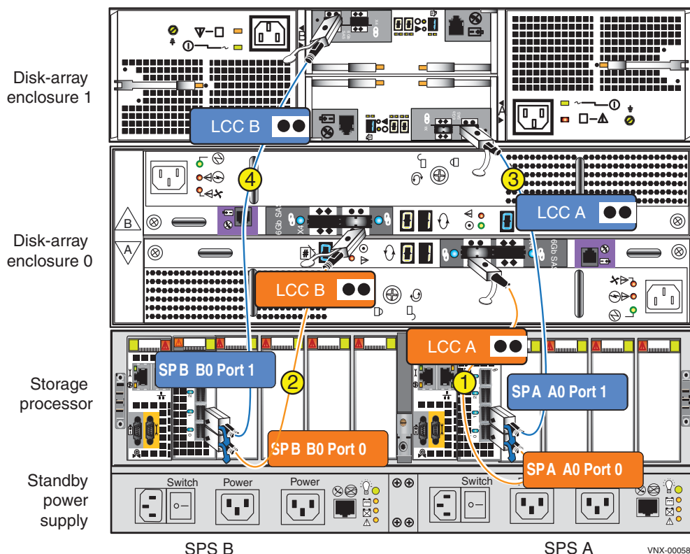
Figure 86 Example of the VNX5700 Block platform with two DAEs (3U, 15 disks and 2U, 25 disks) cabling
