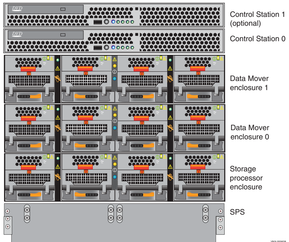
Figure 4 Example of a Block and File (Unified) VNX5700 platform using a 2U SPS (front view)
