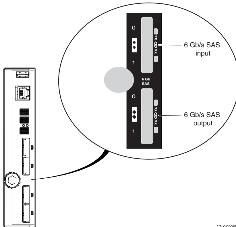
Figure 81 6-Gb/s SAS connectors and LEDs
