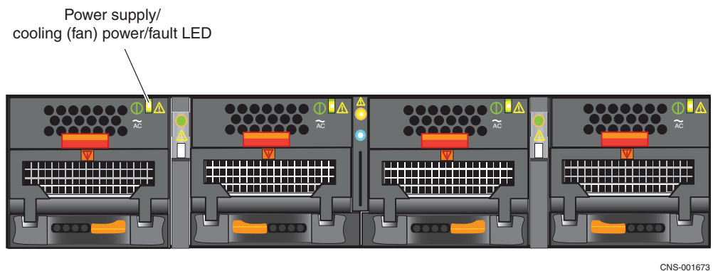
Figure 8 Power supply/cooling (fan) module LED
