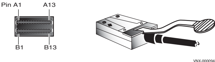
Figure 58 6-Gb/s SAS port and cable connector
