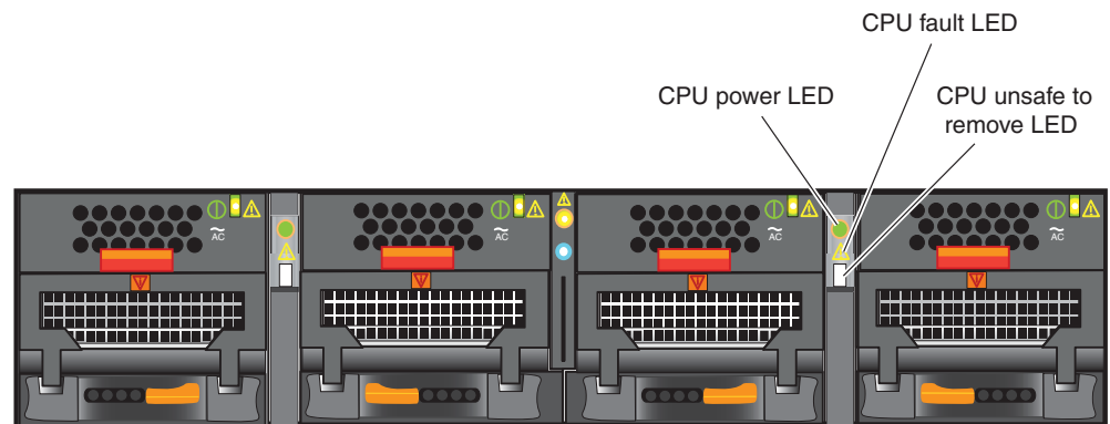
Figure 7 CPU LEDs
