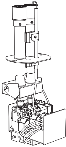
Electronic Burner 34kW
