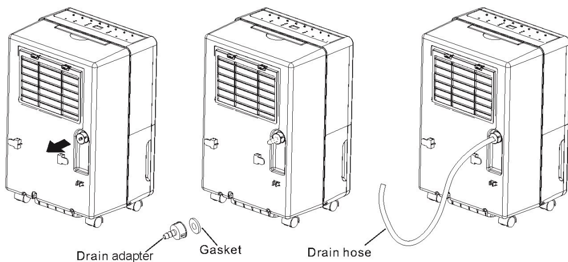
Drain Tube Adapter Storage Compartment
