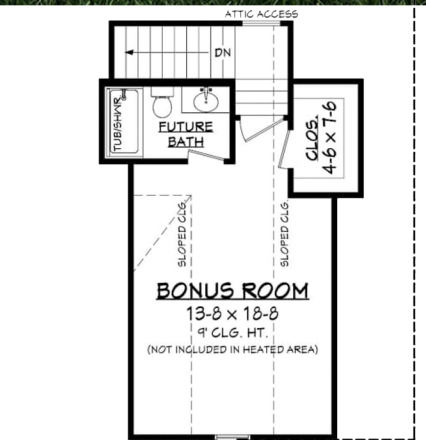
Bonus Floor Plan
