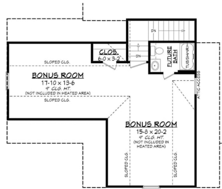
Bonus Floor Plan
