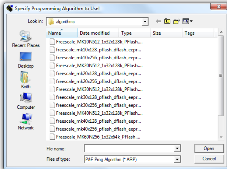
Figure 5-7: Select Algorithm
