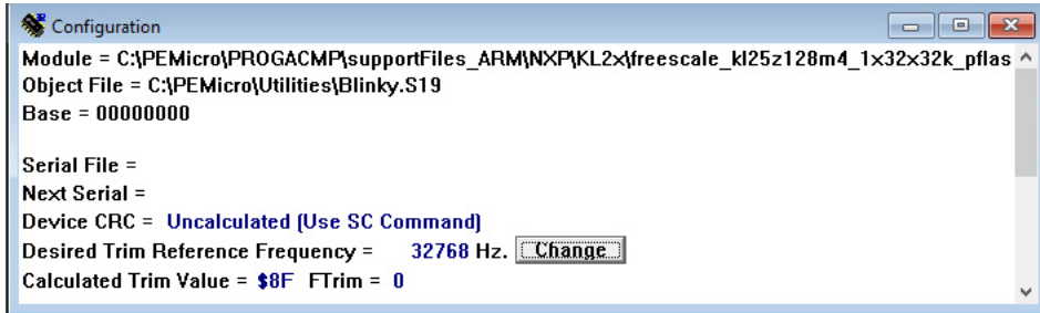
Figure 2-1: Configuration Window
