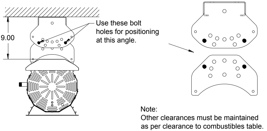
Minimum Ceiling Mount Distance using Optional Shield
