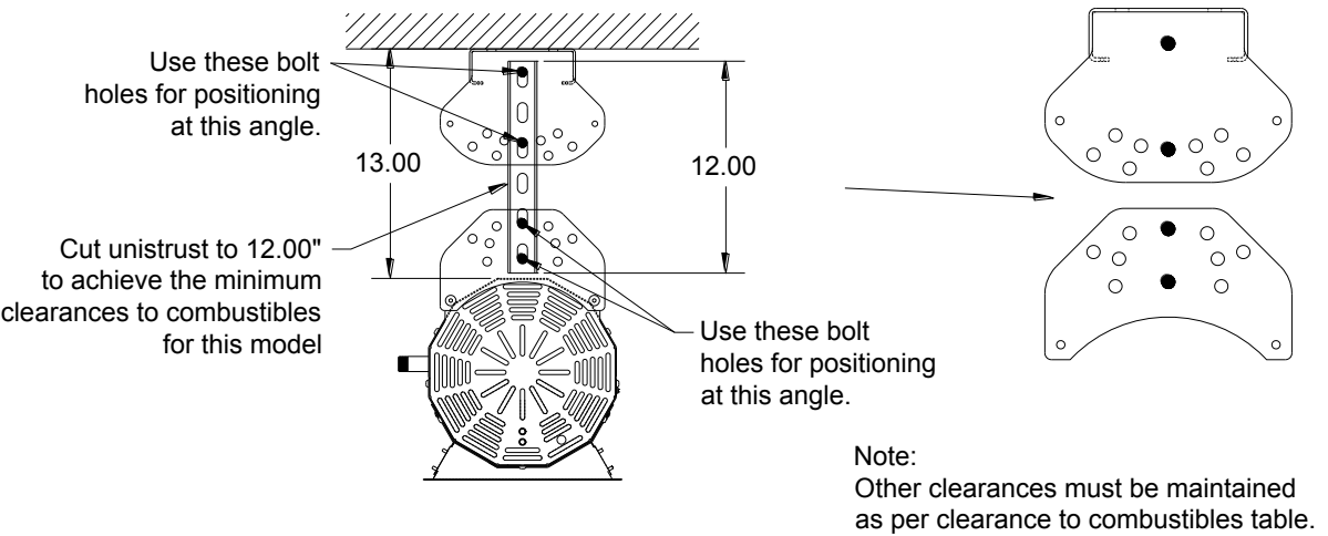
Minimum Ceiling Mount Distance using Optional Shield
