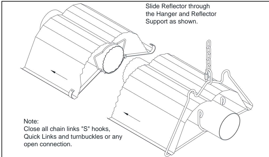
Figure 12: Reflector Installation
