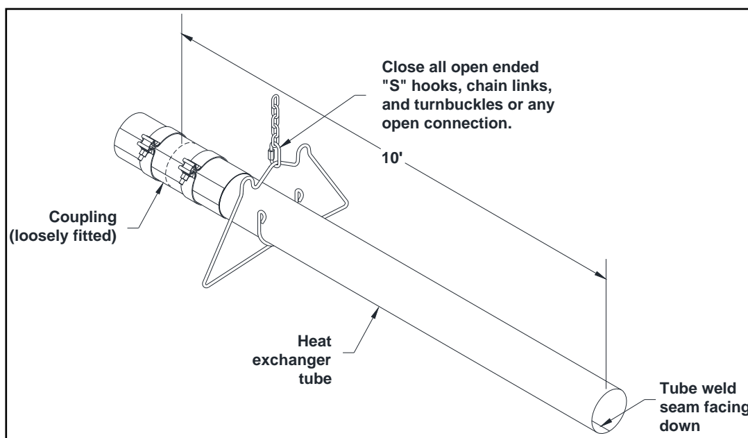
Figure 7: Installation of Heat Exchanger Tube and Coupling
