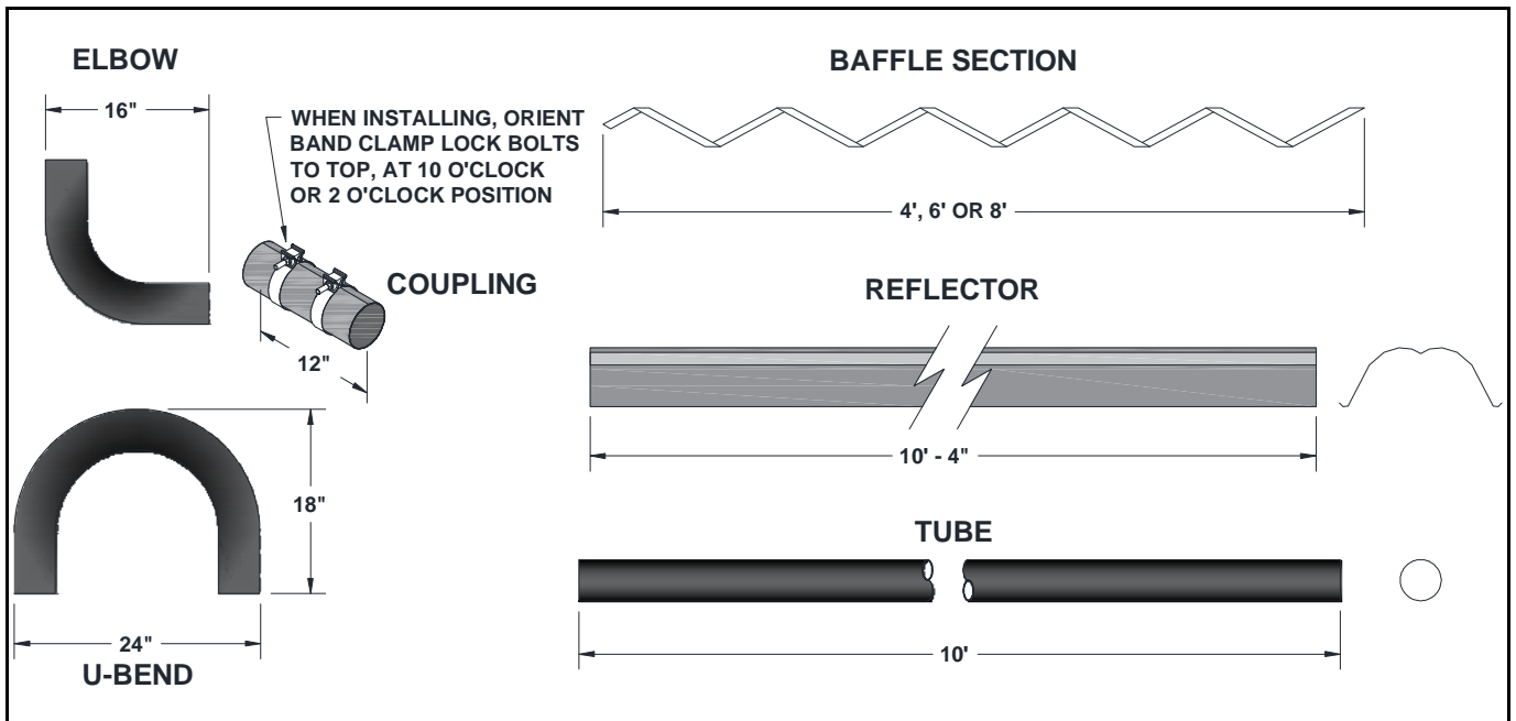
Figure 2: Component Dimensional Information
