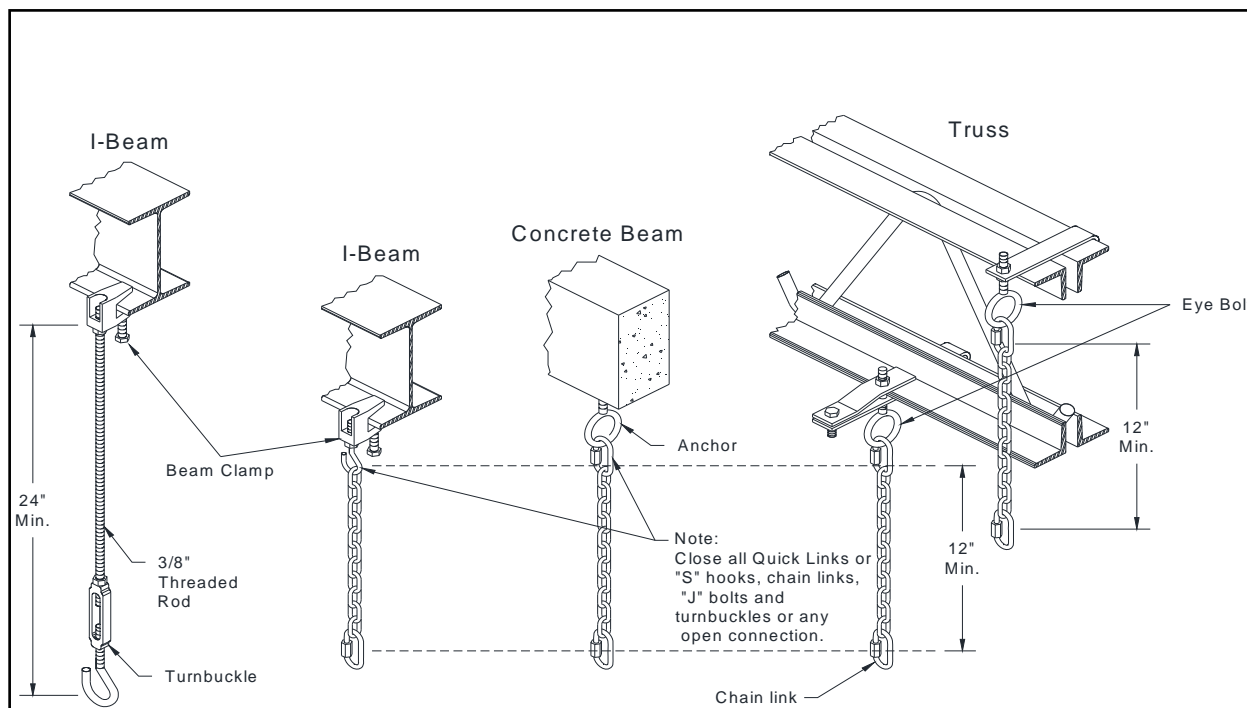
Figure 4: Suspension Mechanism
