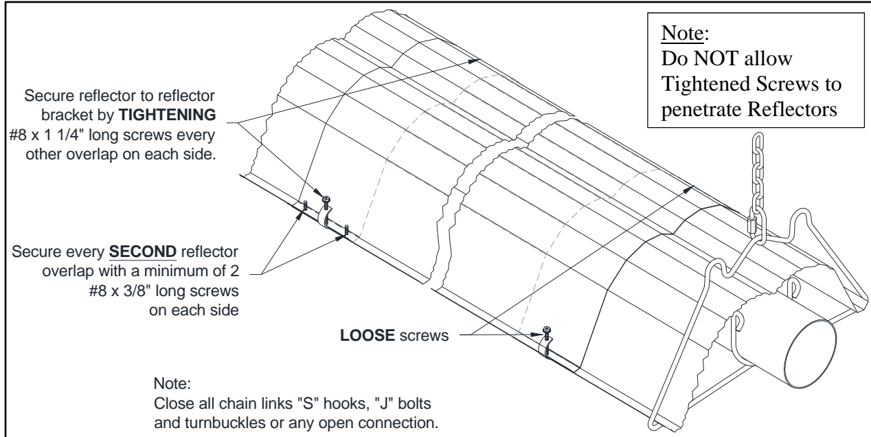
Figure 15: Reflector Supports Installation and Reflector Overlap
