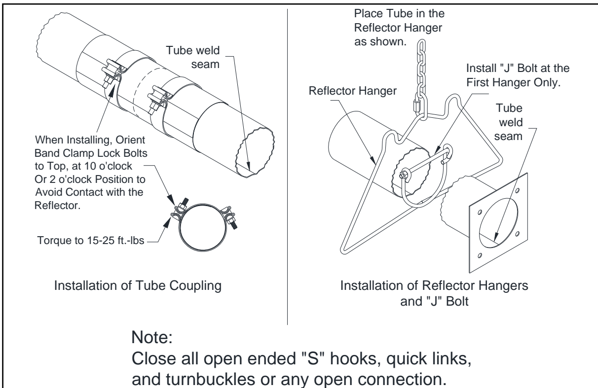
Figure 8: “J” Bolt and Coupling Installations
