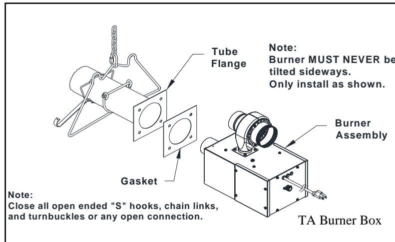
Figure 9: Burner Gasket Installation
