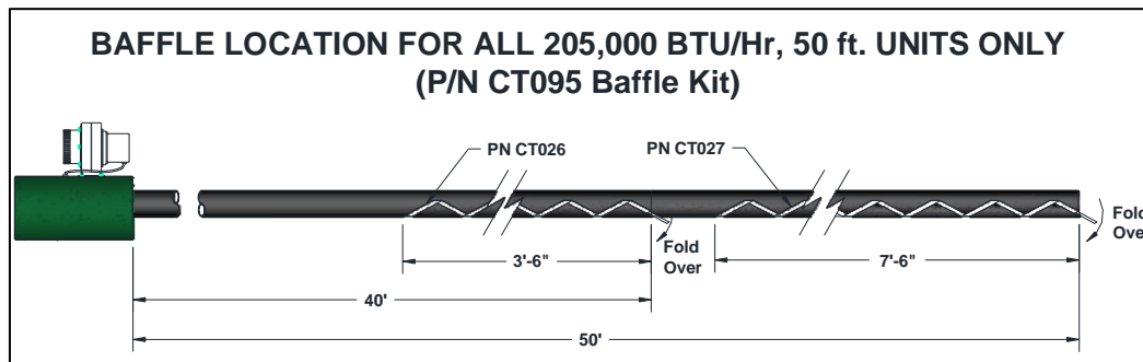
Baffle Location TA/TX/TXR-205 Models, 50ft
