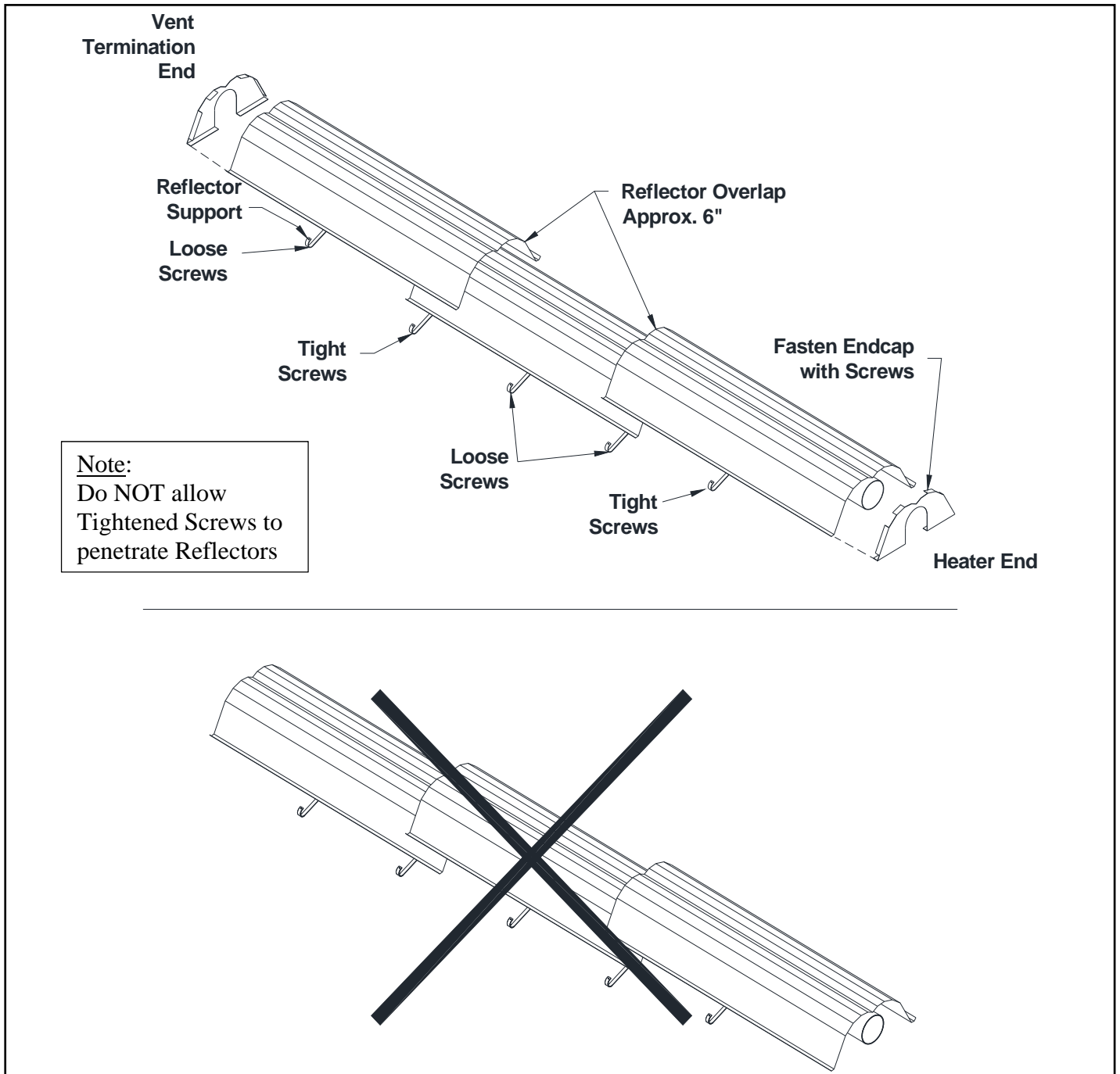
Figure 14: Reflector Overlap Illustration
