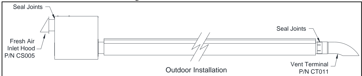
Figure 27: Outdoor Installation
