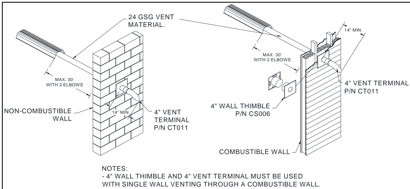
Figure 23: Horizontal Venting
