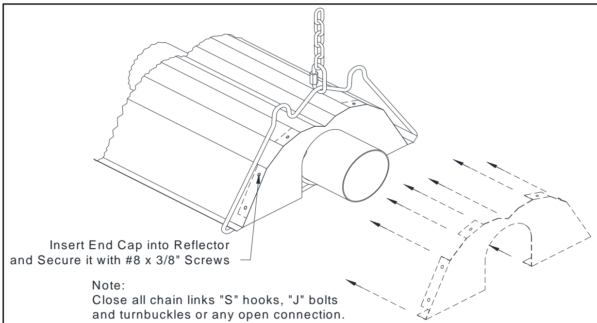
Figure 16: Reflector End Cap Installation
