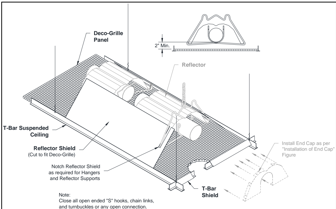
Figure 22: Deco Grille with Suspended Ceiling Installation
