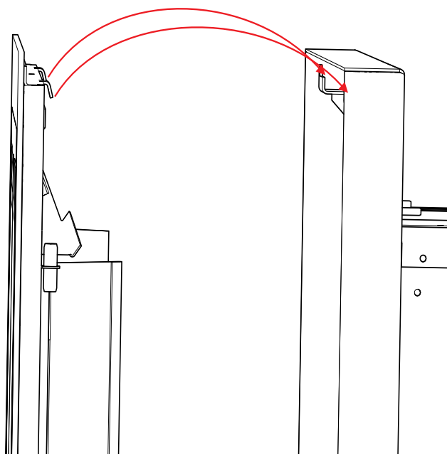
Front Faceplate Install
