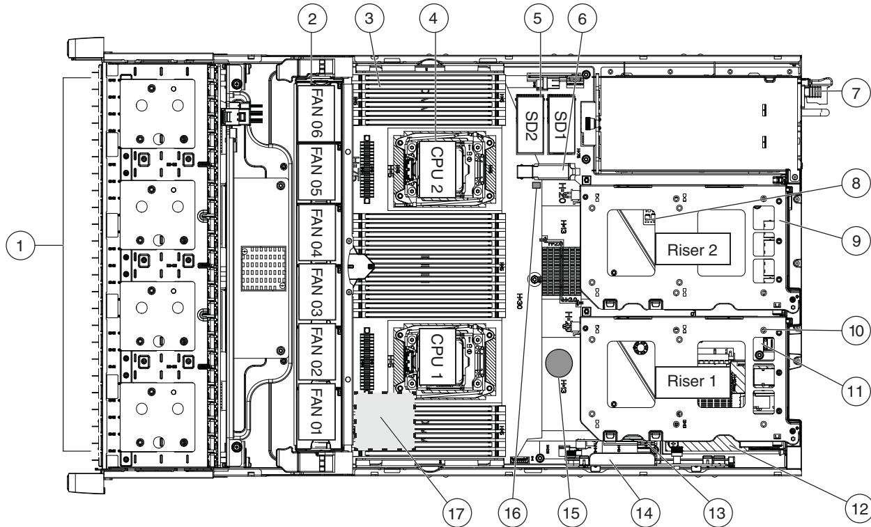
Figure 7 C240 M4 LFF With Top Cover Off
