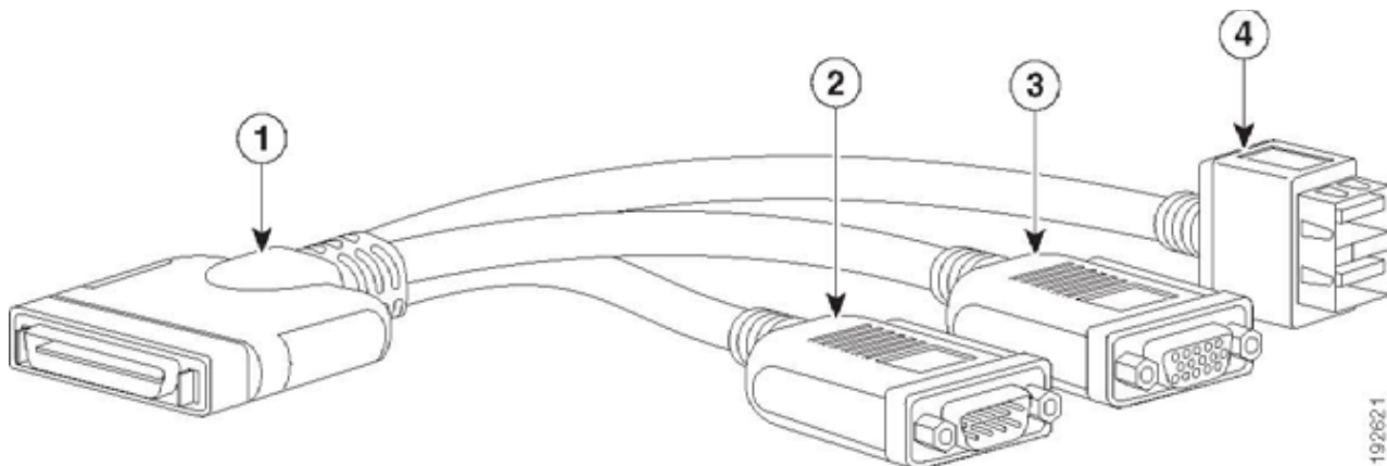
Figure 20 KVM Cable
