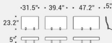
Schienali / Backrests
