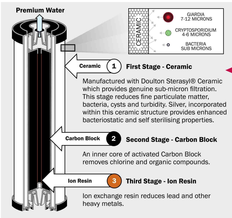
Diagram 2 - The Doulton Ultracarb®
