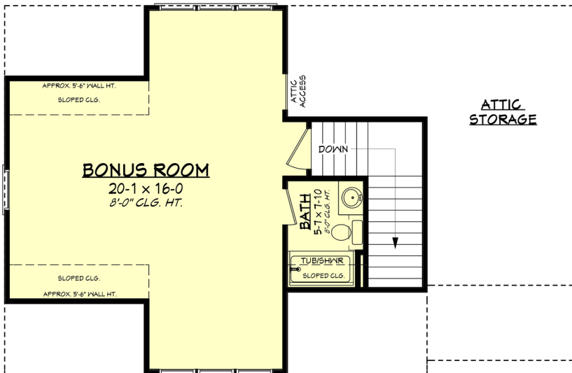
Bonus Floor Plan
