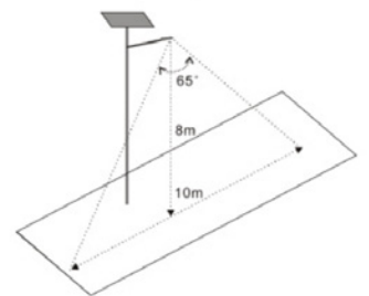
Microwave Sensor
