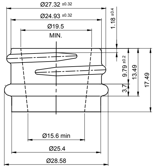
NECK FINISH DETAILS SCALE - 2:1 GPI 28mm-400
