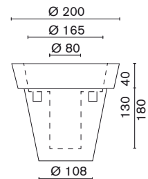
Big-Bo container light
