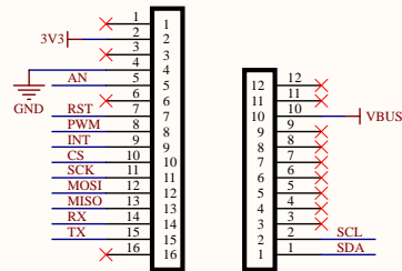
Feather Socket
