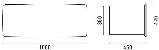
YSCT1A4FD1 Storage element 1060x420
