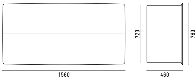
YSCT1A7FD1 Storage element 1560x780
