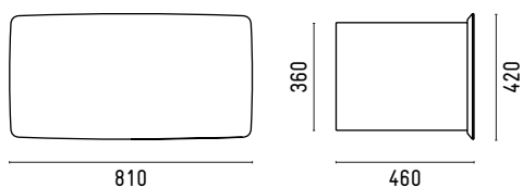
YSCT2 Storage element 810x420
