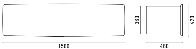
YSCT6 Storage element 1560x420
