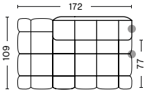
411 | CHAISE LONGUE MODULE | RIGHT WIDTH 172 CM DEPTH 109 CM HEIGHT 72 CM SEAT HEIGHT 41 CM SEAT DEPTH 77 CM
