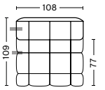
501 | NARROW MODULE | RIGHT W/O ARMREST WIDTH 108 CM DEPTH 109 CM HEIGHT 72 CM SEAT HEIGHT 41 CM SEAT DEPTH 77 CM
