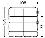
502 | NARROW END MODULE | LEFT W/O ARMREST WIDTH 108 CM DEPTH 109 CM HEIGHT 72 CM SEAT HEIGHT 41 CM SEAT DEPTH 77 CM
