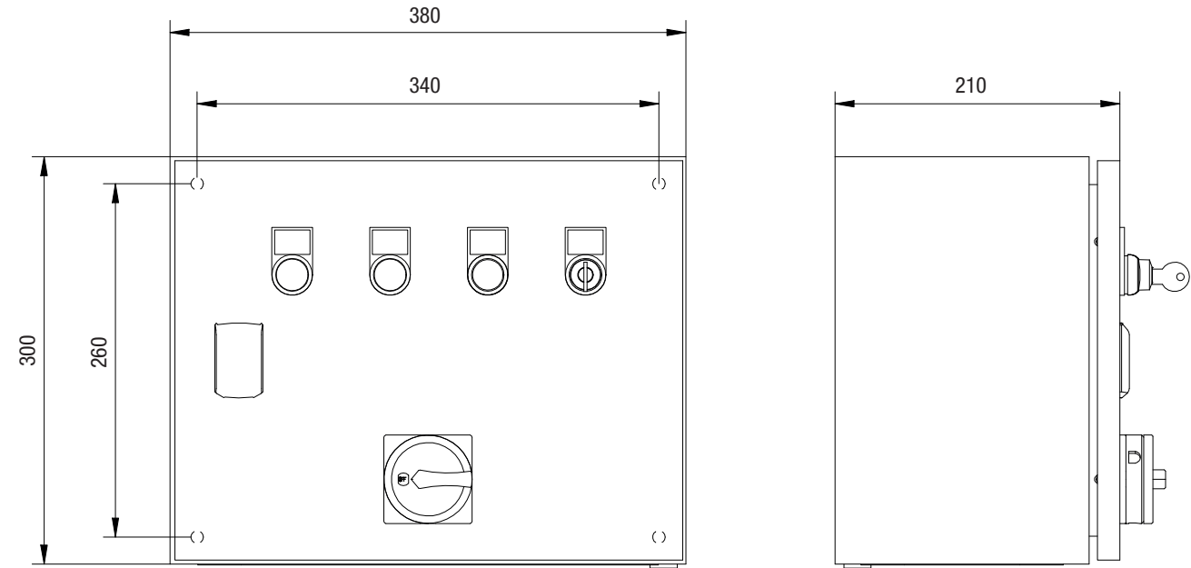
Fig. 3: Dimensional drawing
