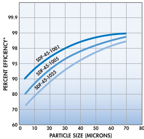
4.5" DIAMETER x 9 3/4" LENGTH
