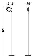
Marselis Floor Lamp
