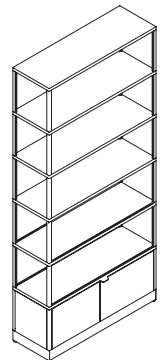
COMBINATION 601 W100 x D34 cm x H220,9 cm
