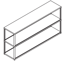
COMBINATION 202 W150 x D34 cm x H74 cm
