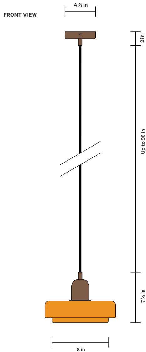
FRONT VIEW
