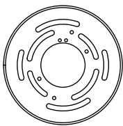
Part A Backplate
