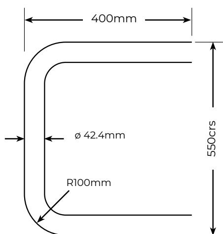
Platform Return Bends 42.4mm diameter from stock
