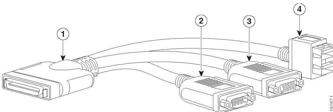
Figure 14 KVM Cable
