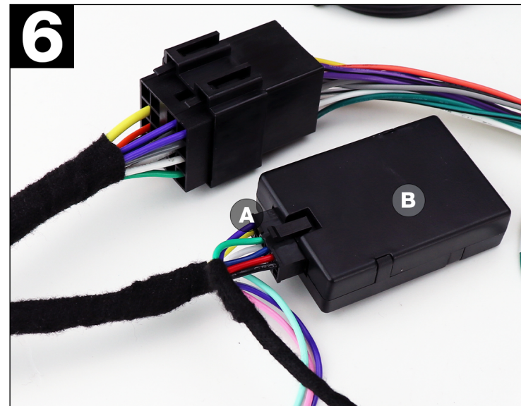
6 ISO connector and CAN interface. Plug the 12 pin molex (A) in to the CAN interface (B) and plug the ISO (male) connector from the CAN104-LR01 harness in to the UN1810E Power lead (ISO female)
