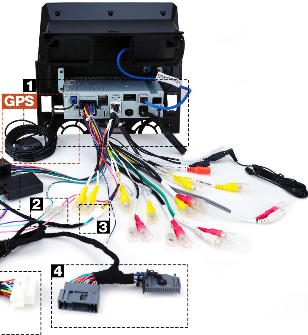
2 CAN signal output wires CAN interface leads: Purple (REVERSE SW), Green (PARKING SW), Pink (SPEED SEN)
