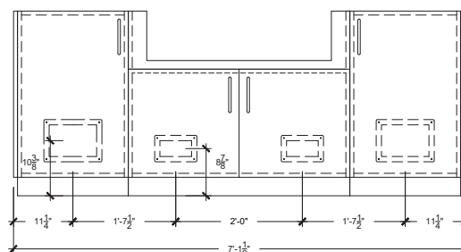
FRONT VIEW (Gas & Electrical Conduits Access Points)
