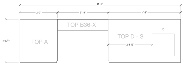
COUNTERTOP TEMPLATE
