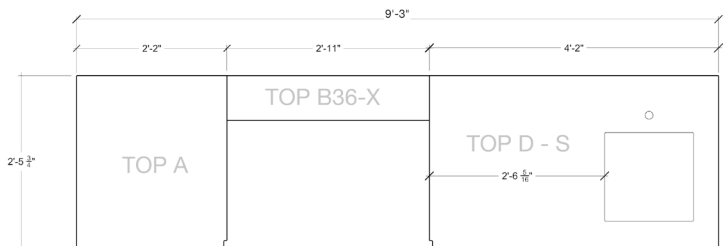
COUNTERTOP TEMPLATE
