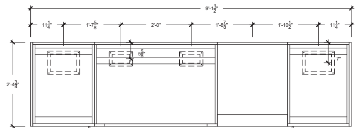
TOP VIEW (Gas & Electrical Conduits Access Points)
