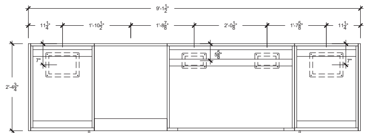
FRONT VIEW (Gas & Electrical Conduits Access Points)
