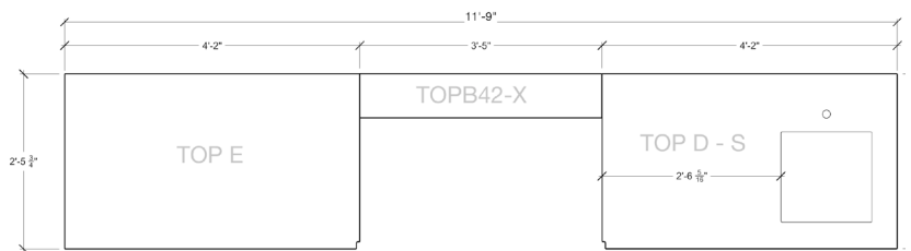
COUNTERTOP TEMPLATE
