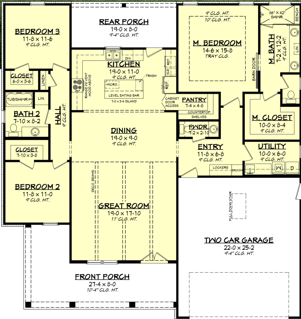
Floor Plan
