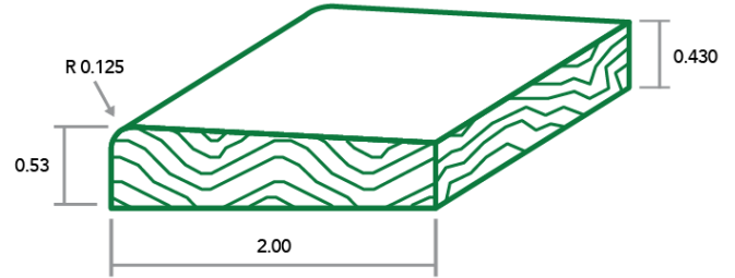
Type "B" Bi-Level Reducer
