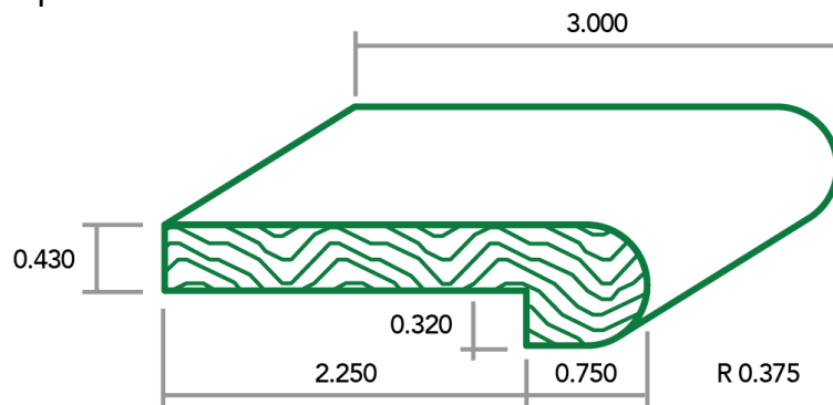
Flush Bullnose Stair Nosing
