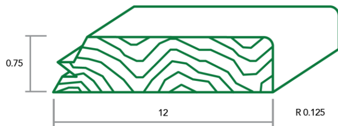
Stair Tread – Square Profile
