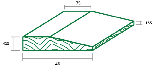
Type "A" Flush Reducer
