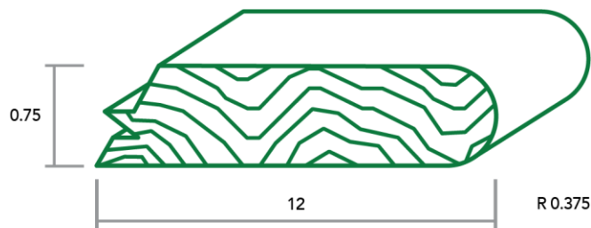
Stair Tread – Bullnose Profile
