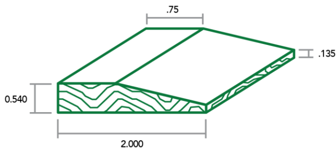
Type "A" Flush Reducer
