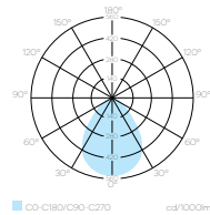
light distribution - down
