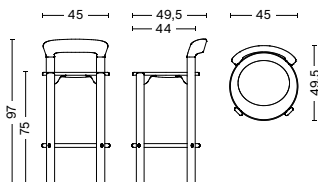
REY BAR STOOL WIDTH 45 CM | 17.72" DEPTH 49,5 CM | 19.5" HEIGHT 97 CM | 38.2" SEAT HEIGHT 75 CM | 29.53" SEAT DEPTH 44 CM | 17.32"
