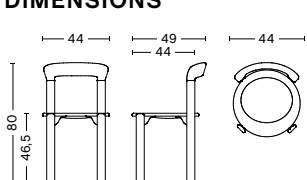
REY CHAIR WIDTH 44 CM | 17.32" DEPTH 49 CM | 19.3" HEIGHT 80 CM | 31.5" SEAT HEIGHT 46,5 CM | 18.31" SEAT DEPTH 44 CM | 17.32"
