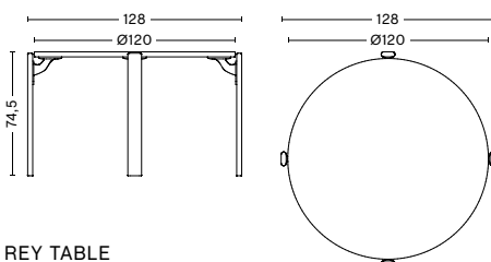
REY TABLE WIDTH 128 CM | 50.4" LENGTH 128 CM | 50.4" HEIGHT 74,5 CM | 29.33" DIAMETER TABLETOP 120 CM | 47.24"
