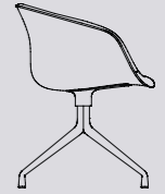
AAC 21 SOFT W59 x D52 x H79/SH46 cm
