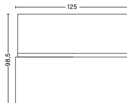
FOLDING CUSHION FOR LOUNGE SOFA WIDTH 125 CM DEPTH 98,5 CM HEIGHT 4 CM
