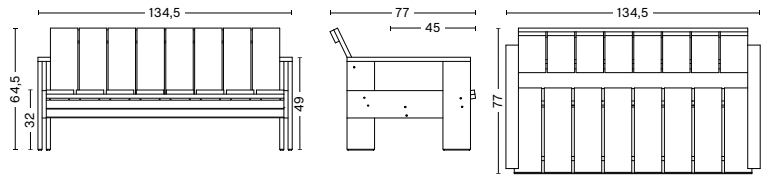
CRATE LOUNGE SOFA WIDTH 134,5 CM DEPTH 77 CM HEIGHT 64,5 CM SEAT HEIGHT 32 CM SEAT DEPTH 45 CM
