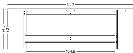
CRATE DINING TABLE L230 WIDTH 230 CM DEPTH 89,5 CM HEIGHT 74,5 CM
