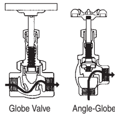
Globe Valve
