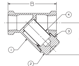
T-221/222-B Threaded
