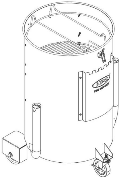
Drum Assembly
