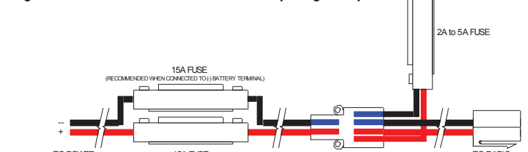
Figure 2 – 40W and 50W Radio Power Cord Splicing Example
