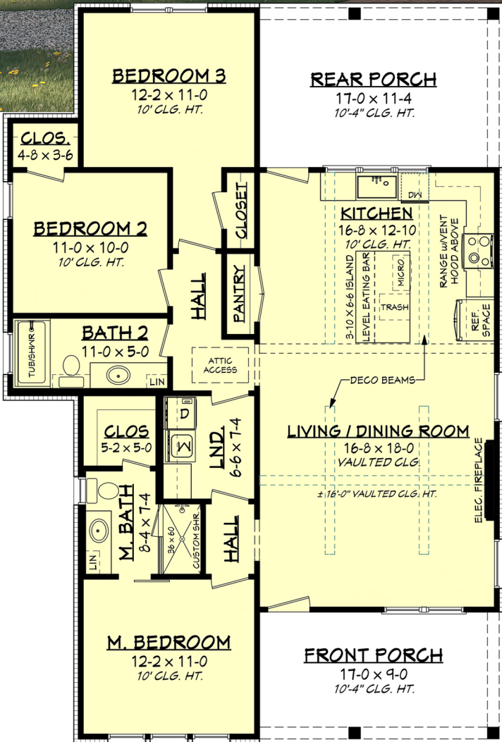
Floor Plan
